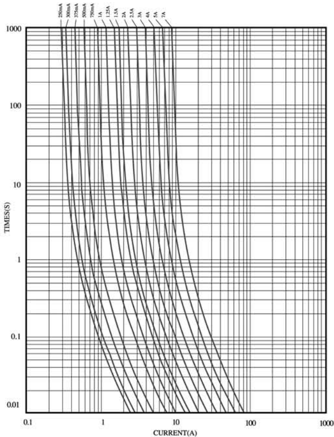
2N RoHS I-T CHARACTERISTICS CURVE 2N RoHS
